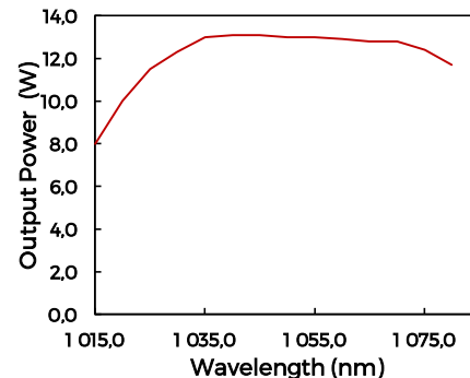
Wavelength tunability from 1020 nm to 1080 nm.
