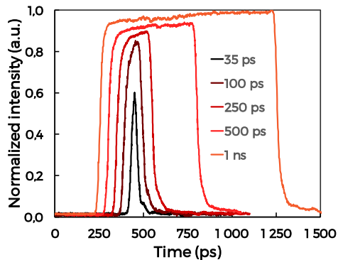
Temporal pulse profile measured with a photodiode from 35 ps to 1 ns.
